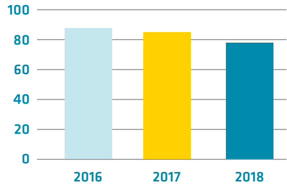
Electrical energy consumption per office area (kWh/m 2 )
